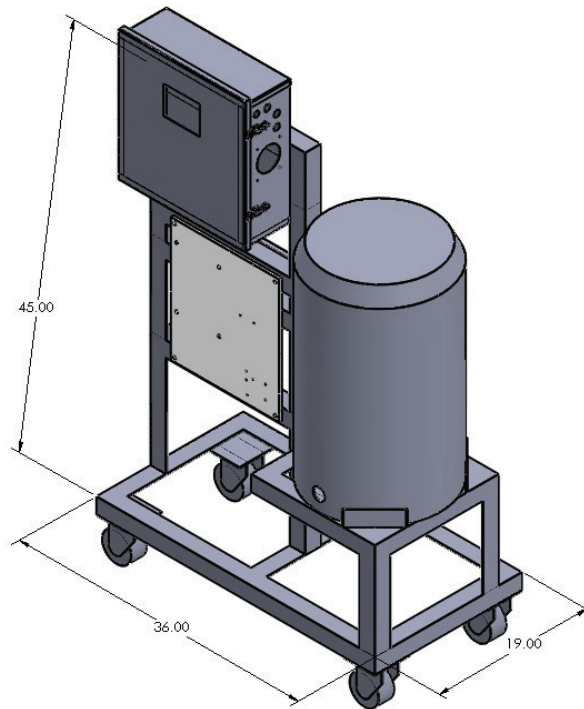
SKID MOUNTED NINJAGEN 360
